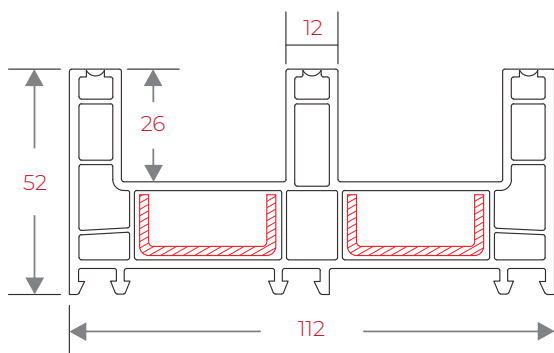
112IRSF52 112 Sliding Frame (3 T)
