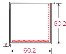
60IRBP1 60 Bay Corner Adaptor
