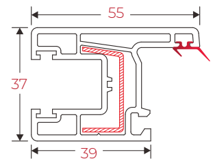
80IRWS55 80 Sliding Window Sash 55
