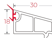
IRCB30 Casement Bead 10mm
