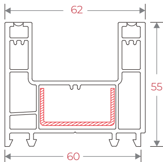
60IRSF55 60 Sliding Frame (2 T)
