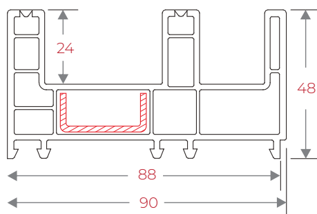
90IRSF48 90 Sliding Frame (2.5 T)
