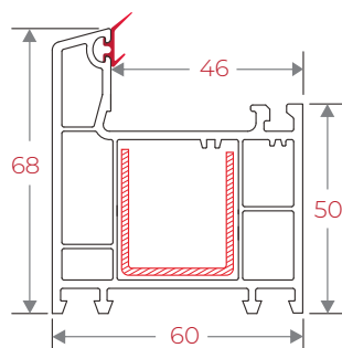
60IRCF68 60 Casement Frame Big
