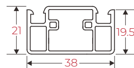
IRMSM Mesh Sash Mullion
