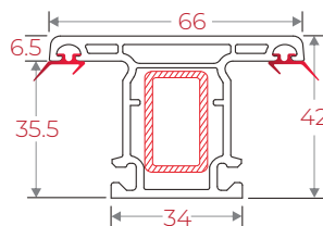
IRSM42 90 Sliding Sash Mullion
