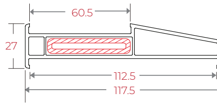
IR11260FB 112/60 Tube Adaptor
