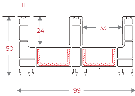
99IRSF50 99 Sliding Frame (3 T)
