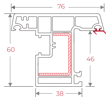
60IRCWS 60 Out Swing Window Sash
