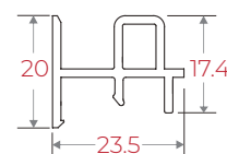
IRMSI Mesh Sash Interlock
