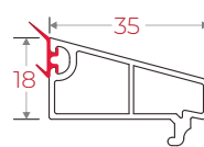
IRCB35 Casement Bead 5mm
