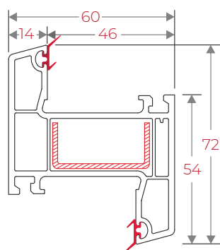
60IRZM 60 Z Mullion
