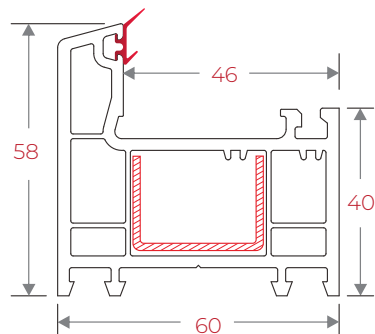
60IRCF58 60 Casement Frame
