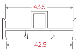
IR42GM 90 Sliding Sash Interlock
