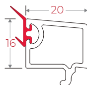
IRSB20 80 Sliding Bead 5mm
