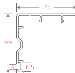
IRSDSC Sliding Door Sash Cover
