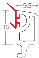
IRSB10 90 Sliding Bead 20mm
