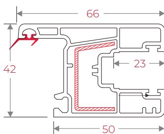
90IRWS66 90 Big Sliding Window Sash 66
