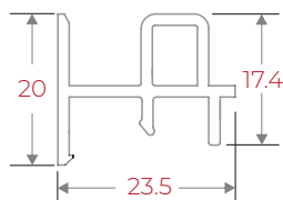
IRMSI Mesh Sash Interlock
