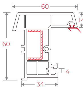
60IRFM 60 Lap Joint
