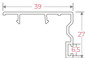
80IRWSC 80 Sliding Sash Cover
