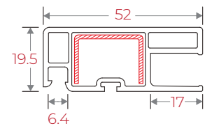
IRMS52 Mesh Sash 52
