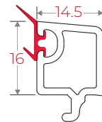
IRSB15 90 Sliding Bead 15mm
