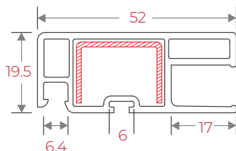
IRMS52 Mesh Sash 52
