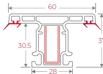
IRSM37 80 Sash Mullion
