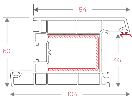
60IRISDS 60 In Swing Door Sash
