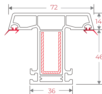
60IRCM 60 Casement Mullion
