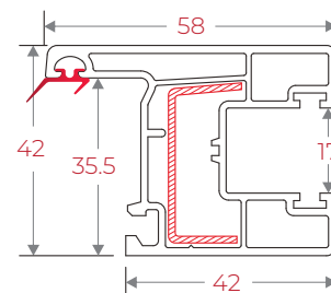
90IRWS58 90 Sliding Window Sash 58
