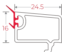
IRSB25 90 Sliding Bead 5mm
