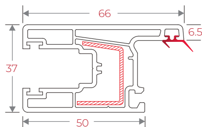
80IRWS66 80 Big Sliding Window Sash 66
