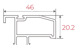
60IRCDSC 60 Casement Door Sash Cover
