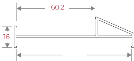
IR9060FB 88-60 Flat Board
