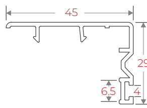
90IRWSC 90 Sliding Sash Cover
