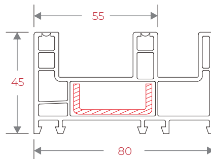
80IRSF45 80 Sliding Frame (2.5 T)
